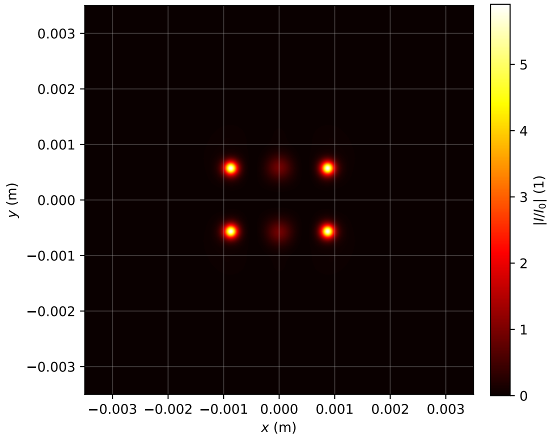
Intensity profile I(x, y, z = 0.876)/I_0 , P_{in}=5.0P_{cr} , artificial time
